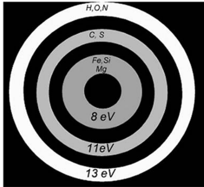
Fig. 5: Elements sorted in a plasma filament in order of their ionization voltage via the Marklund convection process.
