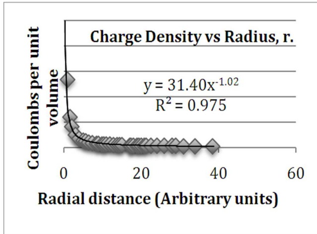
Fig. 3: Charge density produced by the known |j(r)| from the FAC model and the |v(r)| of the observed galaxy from (8).
