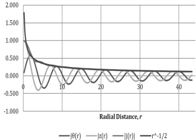
Fig. 1: Current density and its two components. The magnitude of the total current density varies as 1/\sqrt{r} .
