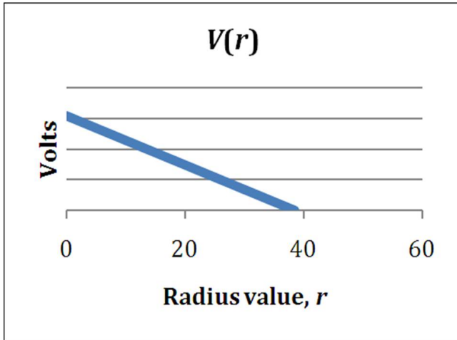
Fig. 4: Voltage profile of cross-section of a FAC.
