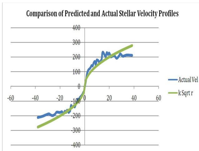
Fig. 6: Comparison of the example galaxy’s measured velocity profile with the Bessel function model’s \sqrt{r} profile.
