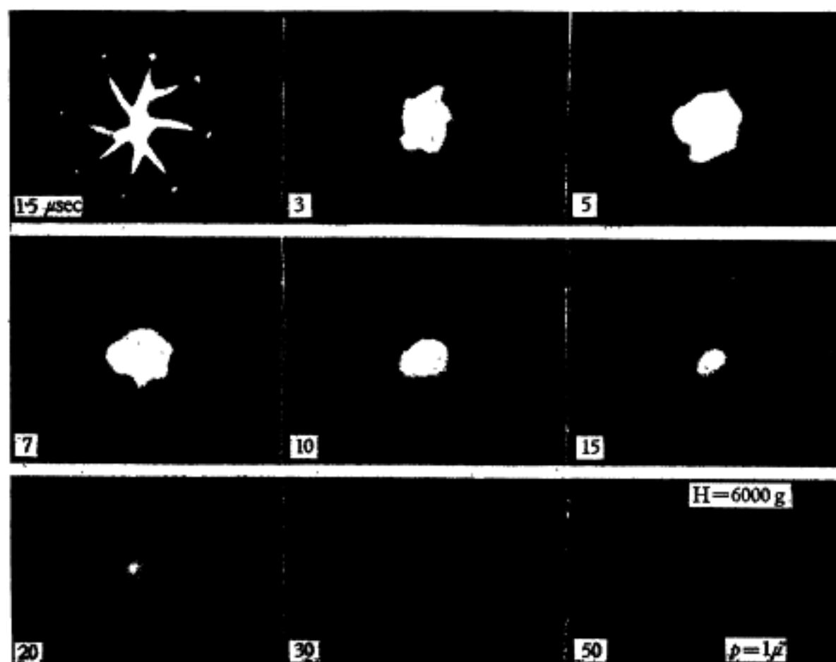
Plate XII. Same as Plate XI except that the sources are aimed to produce an even smaller ring. The original photograph shows an illuminated blob of plasma lasting out to 50 \mu sec.
