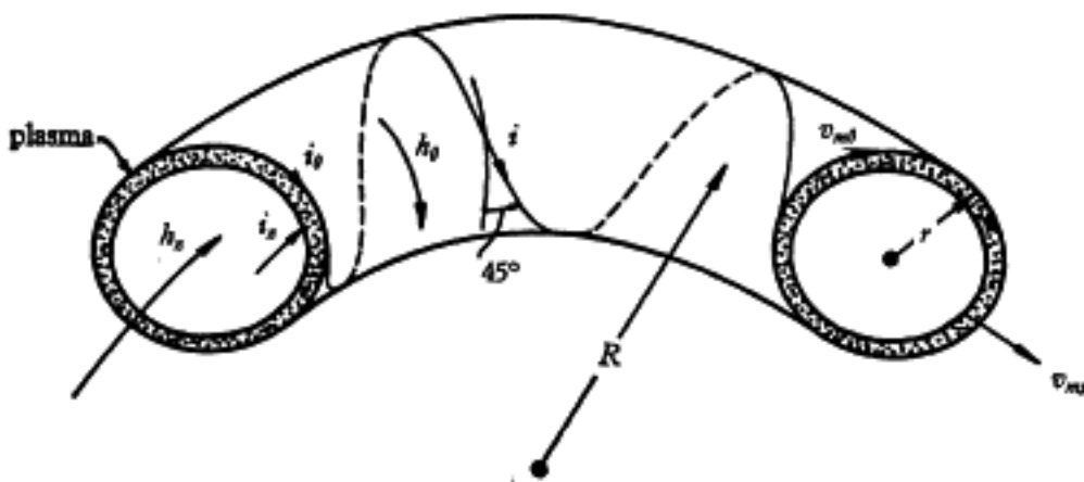
Fig. 1. The S-plasmoid . This configuration of magnetic field and plasma is essentially the same as that of the H -centered pinch in a toroidal tube which was first proposed and investigated experimentally in the United States in 1955 by M. A. Levine and L. S. Combes [Tufts University, Dept. of Physics Report, January 30, 1956 (unpublished)]. The configuration has since received theoretical development by M. N. Rosenbluth and C. L. Longmire [ Annals of Physics , 1 , 120, 1957]. Papers 47-49 of this volume are reports on experimental and theoretical work on the same configuration in a straight tube (see also I. N. Golovin et al. , J. Atomic Energy U.S.S.R. , 5 , 26, 1956; V. D. Shafranov, J. Atomic Energy U.S.S.R. , 5 , 38, 1956).
