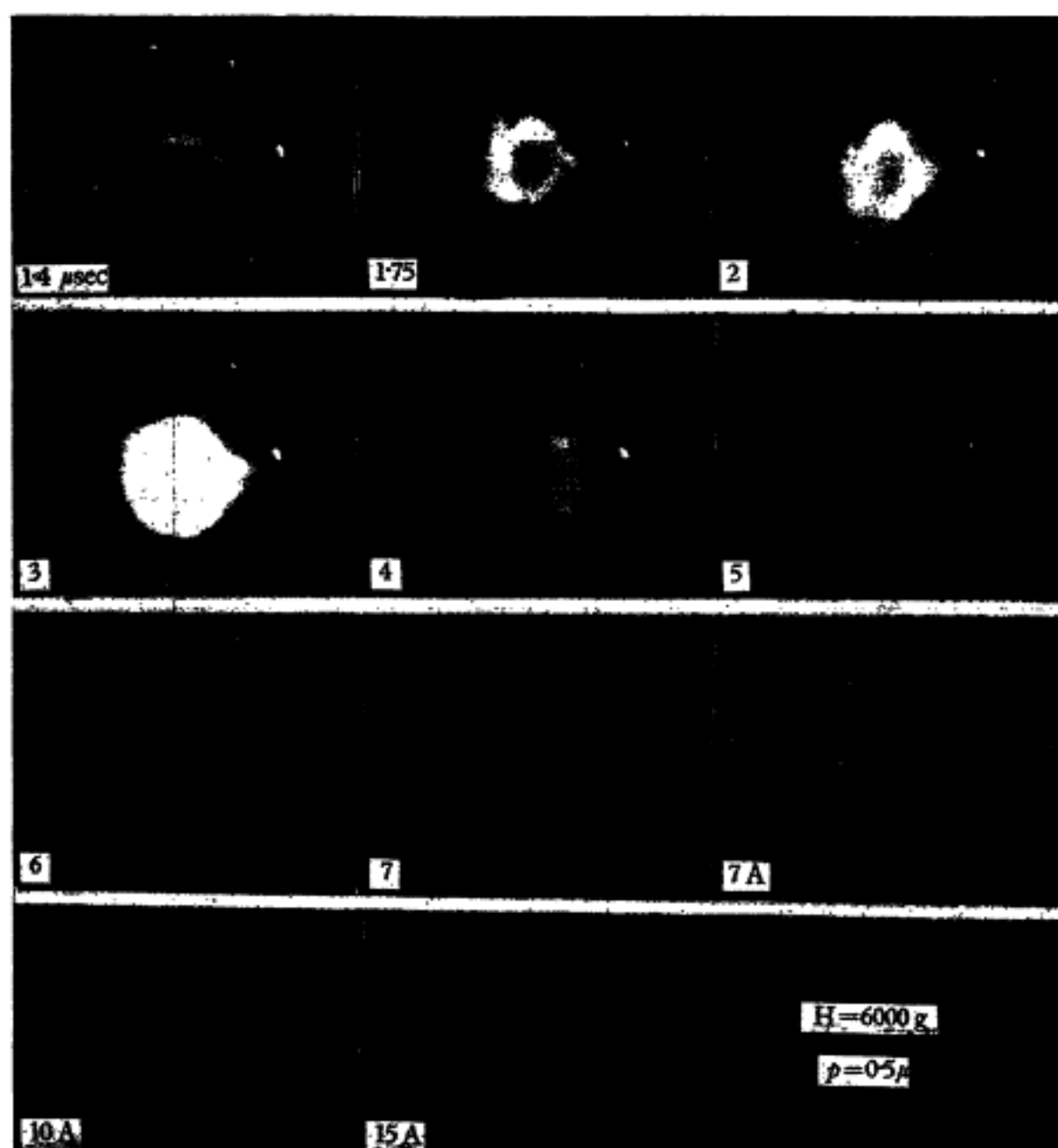
Plate XIII. Sequence of photographs taken in a manner similar to those of Pl. IX except that the source current is in the direction which aids the velocity of propagation of the plasmoid across the magnetic field, and the pressure is 0.5 \mu . The whirl-ring which is formed gets progressively out of focus as it apparently moves toward the camera, and at 7 \mu\text{sec} delay, it is badly blurred. The delay times '7A, 10A, and 15A' correspond to moving the camera back 15 cm which, at least for 7A sharpens up the picture. It is believed that for delays 10A and 15A, and perhaps for 7A, the ring has travelled until it has encountered the lucite window of the vacuum system which is 20 cm from the position where the ring is formed.
