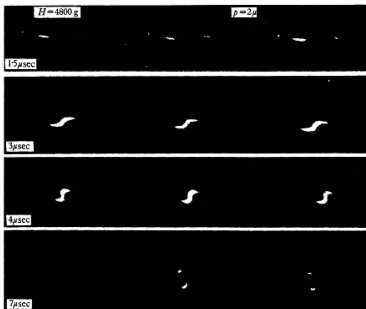
Plate III. A sequential study of barred spirals which are produced by firing two plasmoids from sources 10 cm apart at one another simultaneously across a magnetic field of 4800 gauss. The Kerr cell exposure times are 2 \mu\text{sec} and the various delay times of the sequence are indicated in \mu\text{sec} . The pressure in the chamber is 2 \mu . The plasmoids and their trajectories are rendered luminous primarily by the recombination light of the titanium and deuterium ions which come from the plasma source. The photographs on the left are the left stereo photos and those on the right, the right stereo photos, with an angle between the two views of 10^\circ . The middle photograph is taken straight ahead along the direction of the magnetic field. The current (3000 amperes for 0.4 \mu\text{sec} ) through the source produces a magnetic field which opposes the d.c. field and diminishes the velocity of projection of the plasmoid across the magnetic field.
